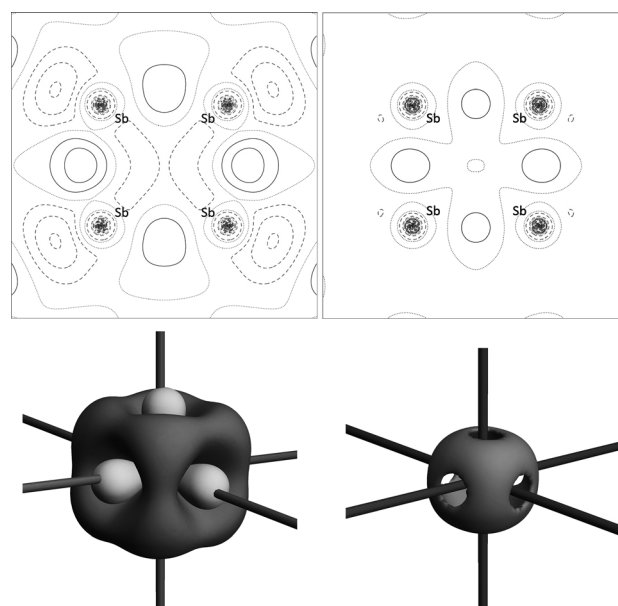
Figure 2. Static deformation density in the plane of the Sb 4 ring from multipole modeling of experimental structure factors (a) and theoretical structure factors (b) with a contour level of \pm 0.05 \text{ e } \text{\AA}^3 (dark-gray: positive, light-gray: zero, dotted: negative). c) Static deformation density isosurface ( \pm 0.25 \text{ e } \text{\AA}^3 ) of the CoSb 6 octahedra for the experimental data. Straight lines represent the directions toward Sb. d) 3D experimental Laplacian distribution of Co at a contour level of -700 \text{ e } \text{\AA}^5 . For c and d, the corresponding plots from theory are shown in the Supporting Information.
